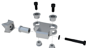
Shown with 2-Piece Tooth
